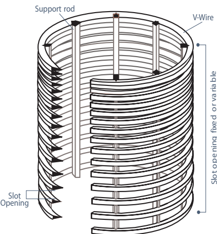
Resistance Welded Wire Screens are manufactured in cylinders and then flattened
