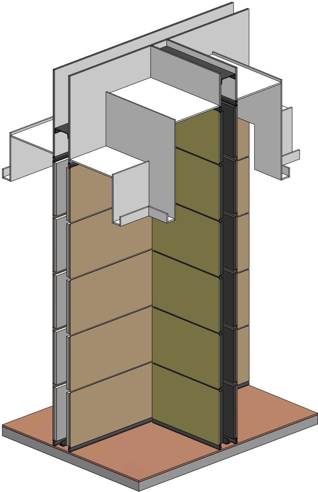
Stacked walls Pocket detail
